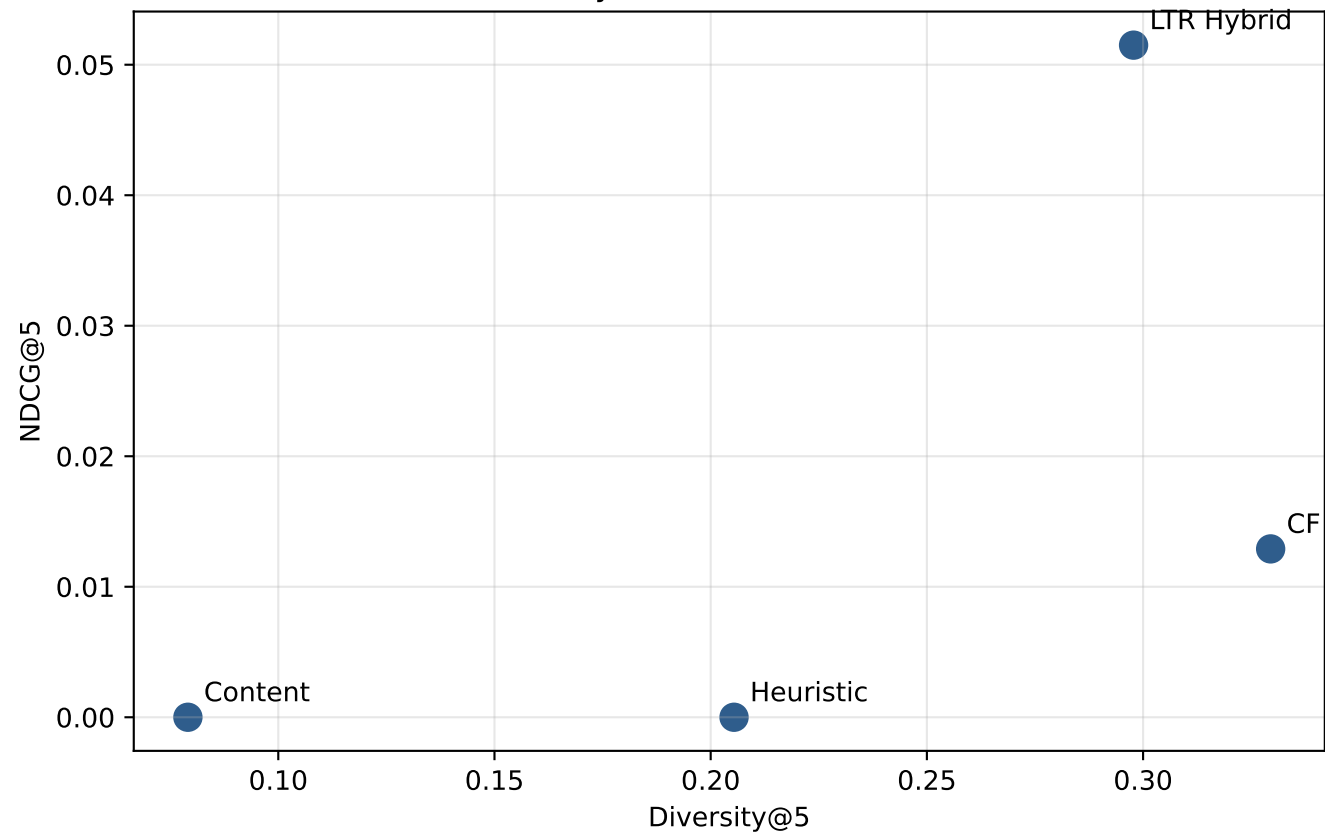
Diversity vs Relevance Trade-off
