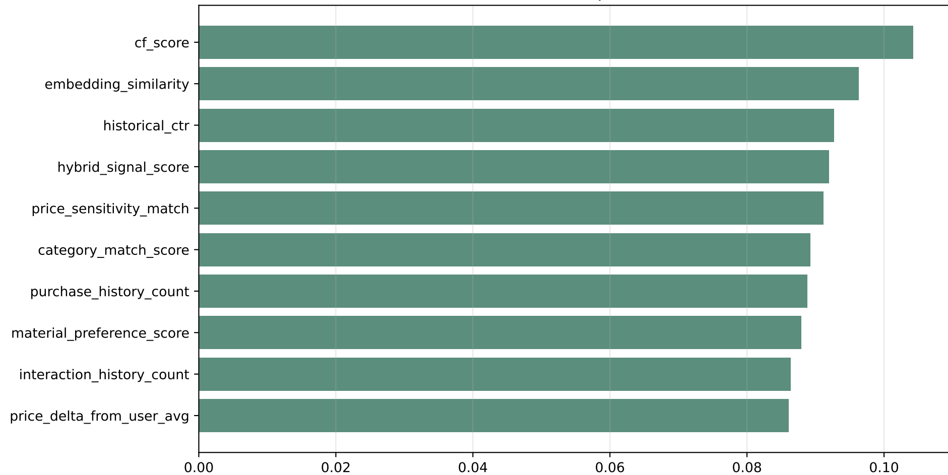
LTR Feature Importance
