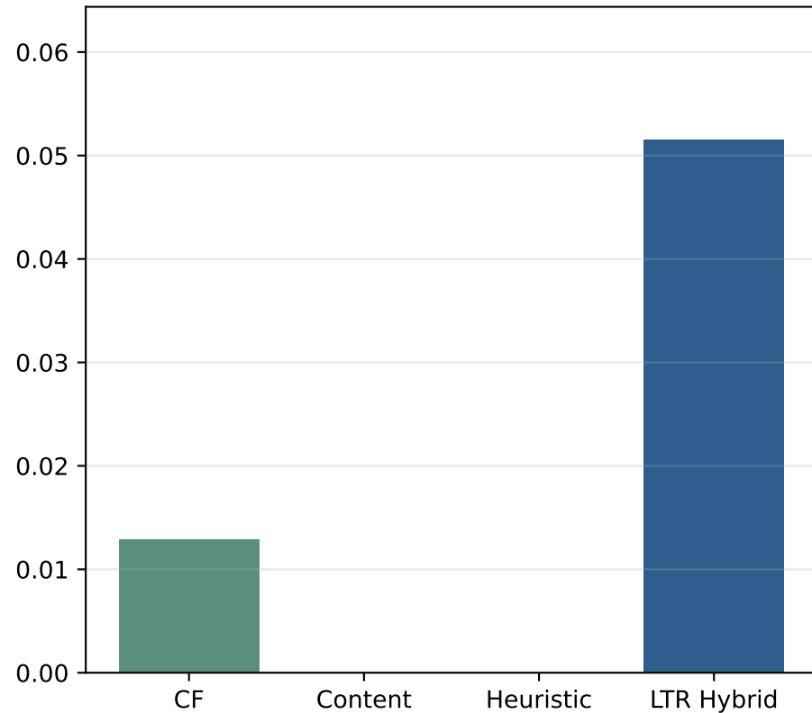
NDCG@5
